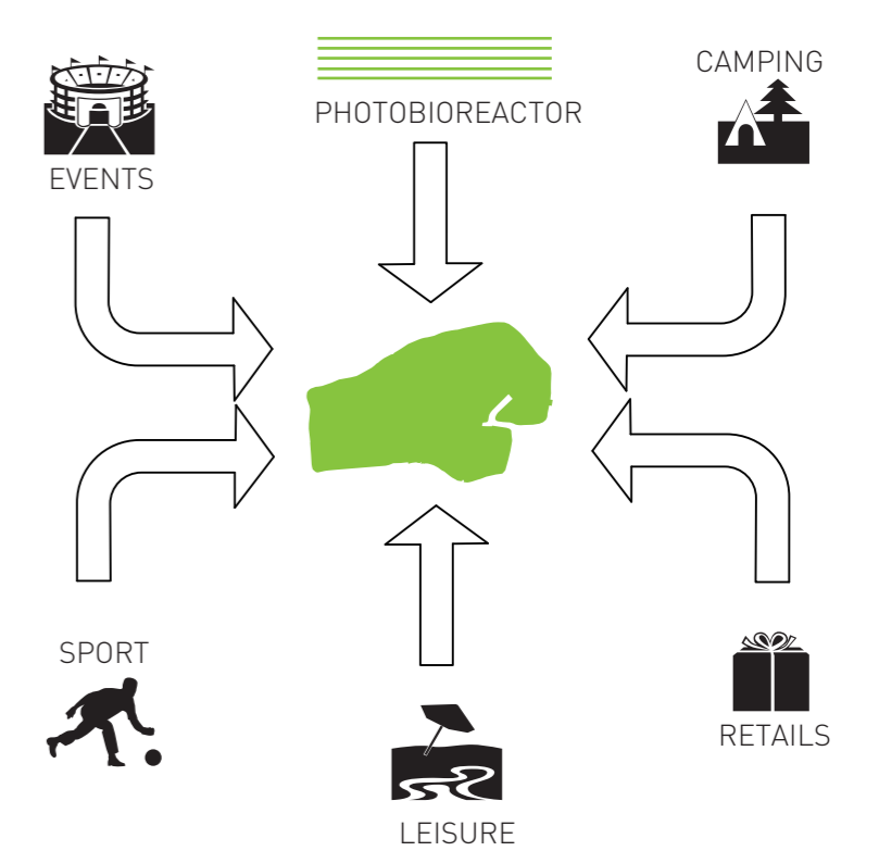
SUPERPOSE USES
